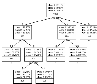
Fig. 2. Hybrid CHAID tree for 11 dependent variables.
