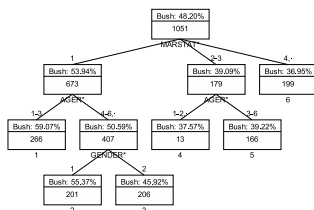
Fig. 3. Hybrid CHAID tree for VOTE.
