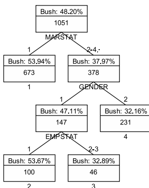
Fig. 1. CHAID tree for VOTE.
